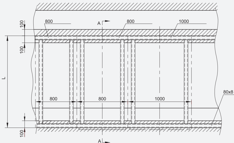
Figure 3/2 Schematic Switchgear Installation Foundation
