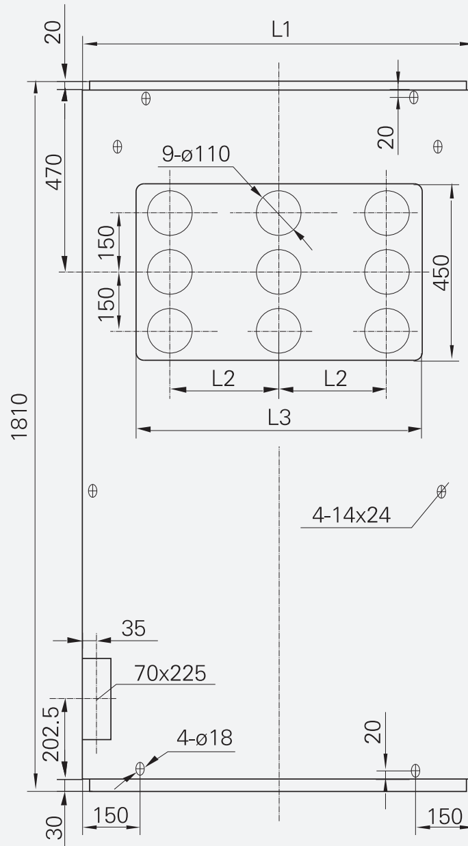
Figure 3/3 Bottom Plate Dimension
